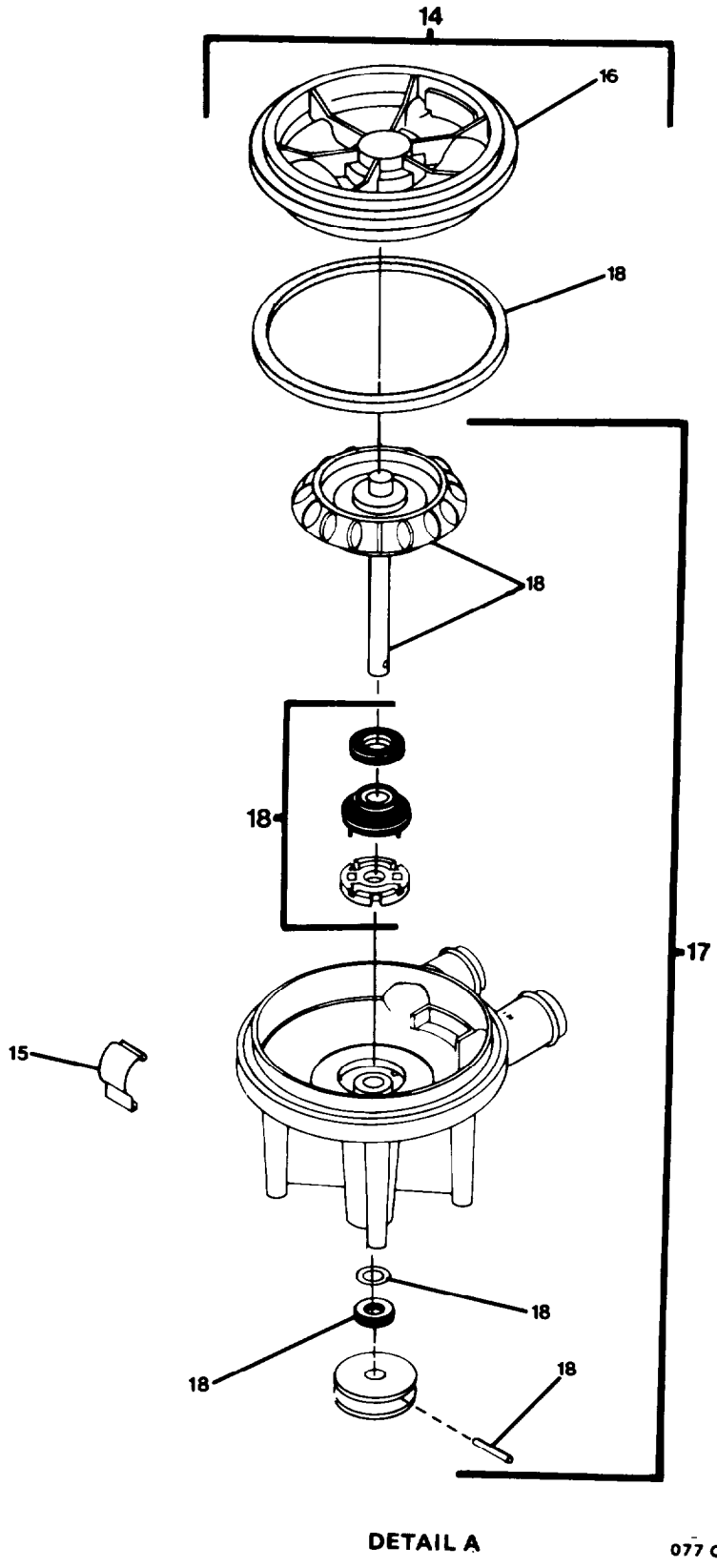
FIGURE 426. Pump Assembly, and Hoses Group (Sheet 2 of 2).
