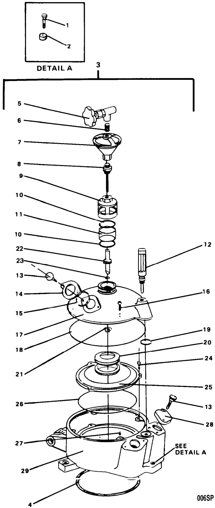
FIGURE 329. Hood Assembly.
