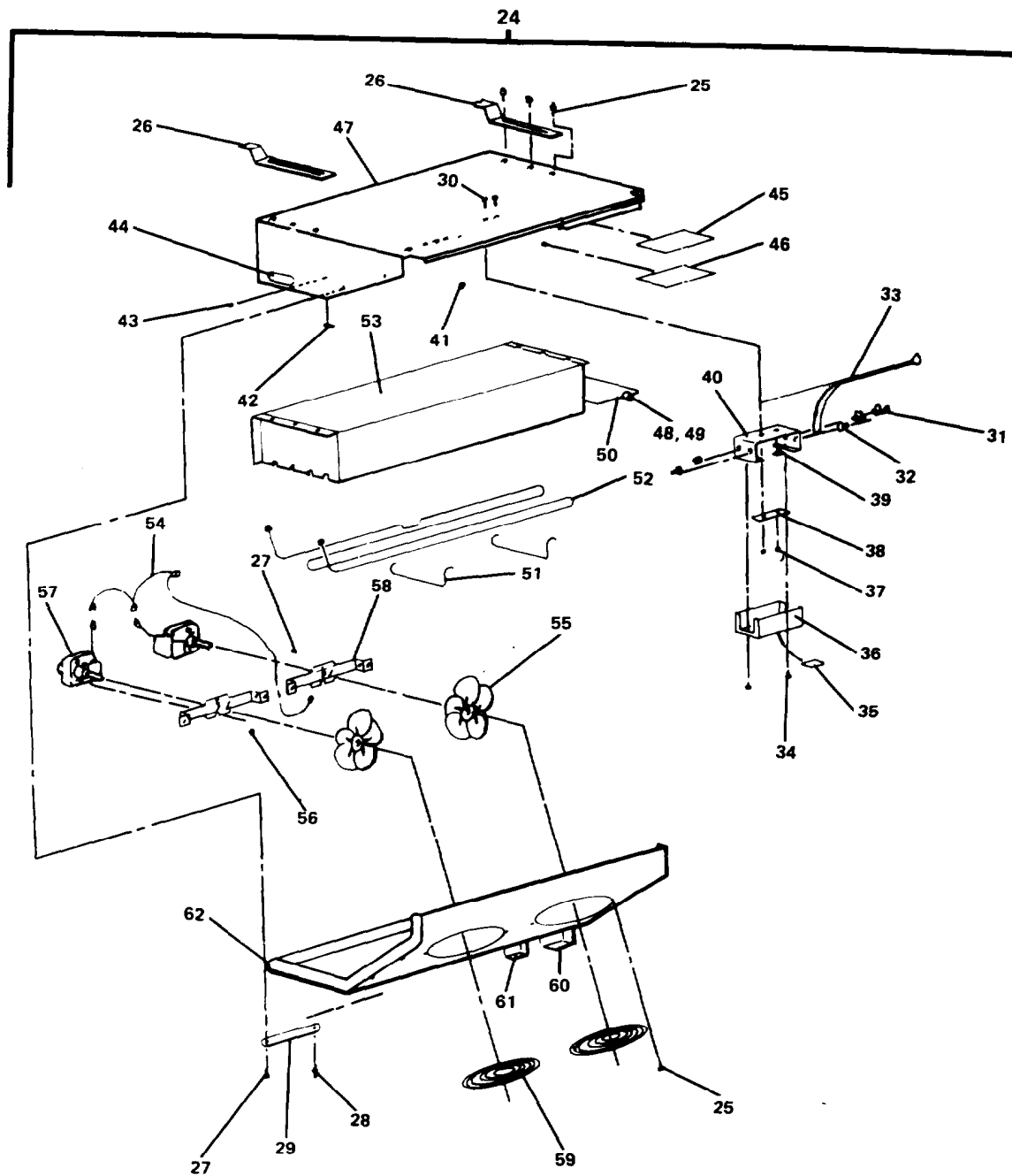
DETAIL A EVAPORATOR COIL ASSEMBLY
