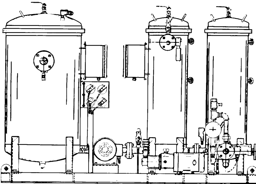
OIL/WATER SEPARATOR
