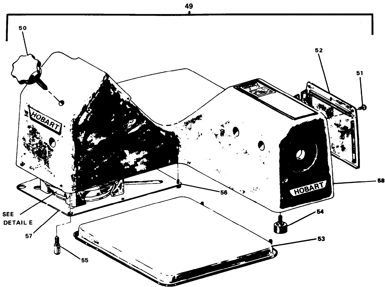
DETAIL D BASE UNIT ASSEMBLY
